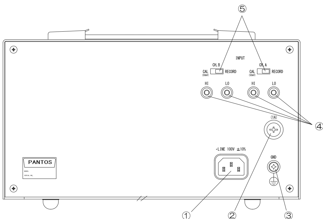
Fig.4.2.1 Rear panel
